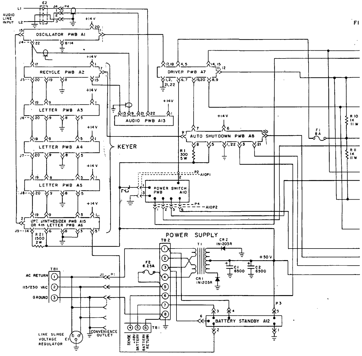
TRANSMITTER SCHEMATIC
