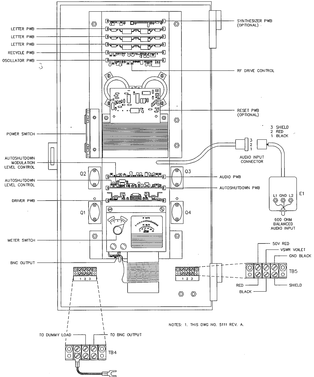
TRANSMITTER DIAGRAM
