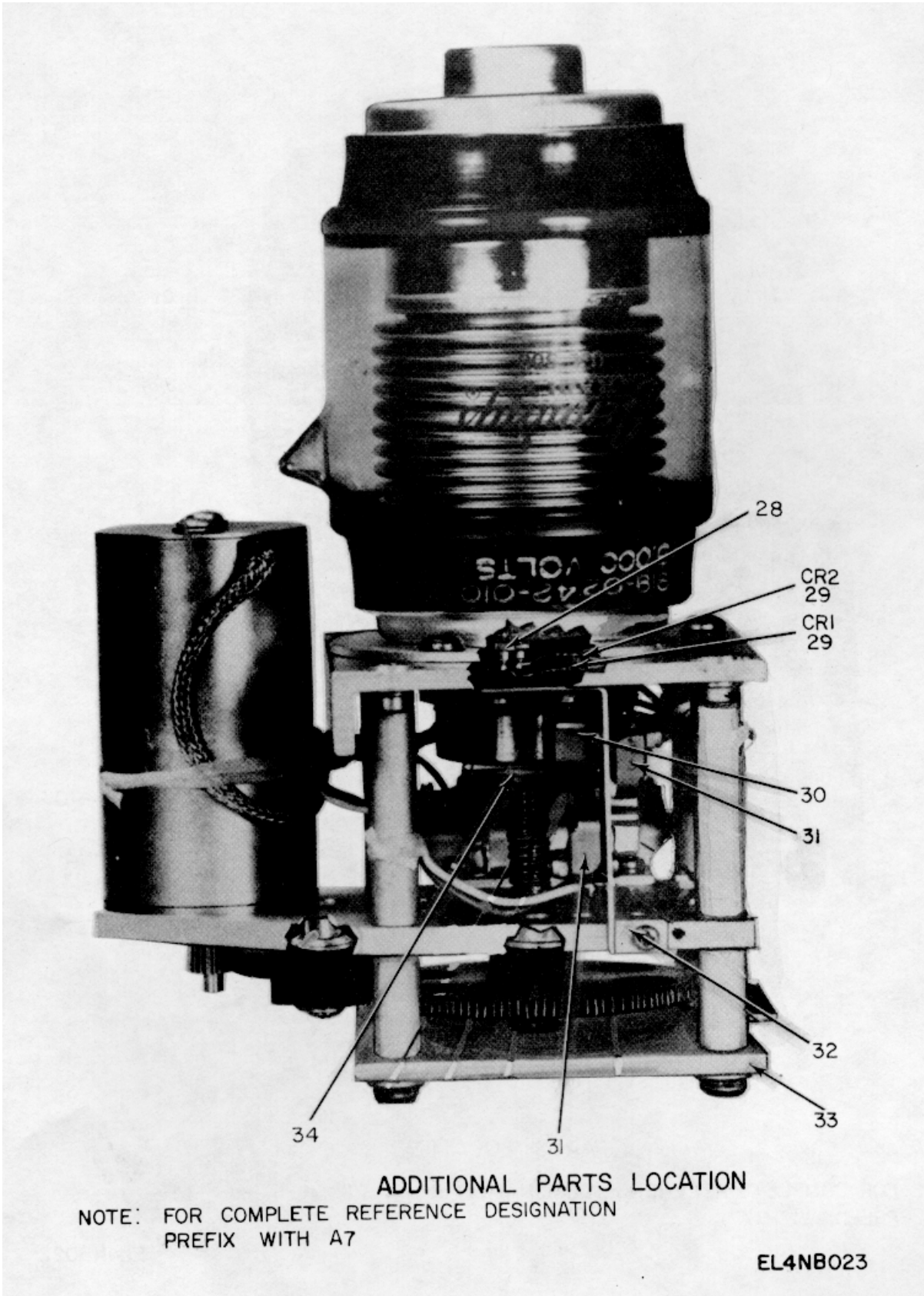
Figure 16. Capacitor Assembly, Variable, RF Shunt (A7) (Sheet 2 of 2).
