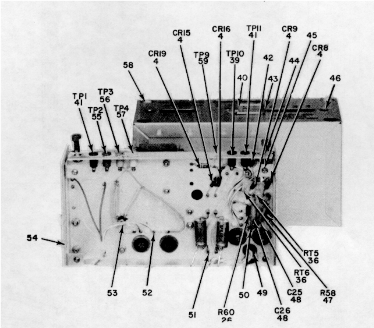
REAR VIEW
