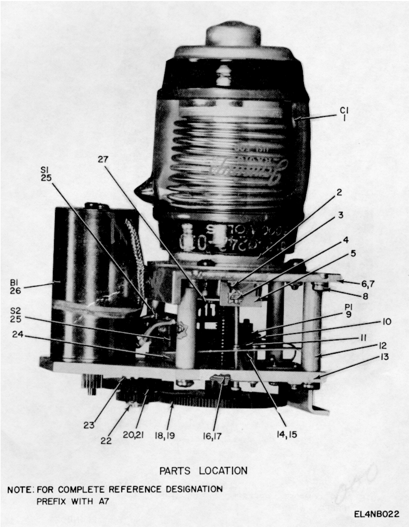
Figure 16. Capacitor Assembly, Variable, RF Shunt (A7) (Sheet 1 of 2).
