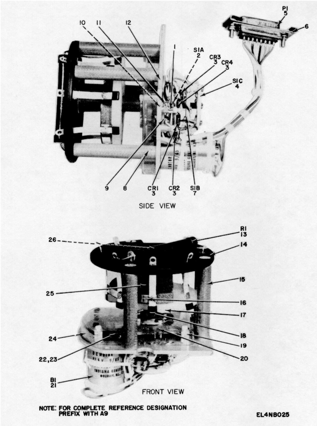
Figure 18. Capacitor Assembly, Variable, RF Series (A9).
