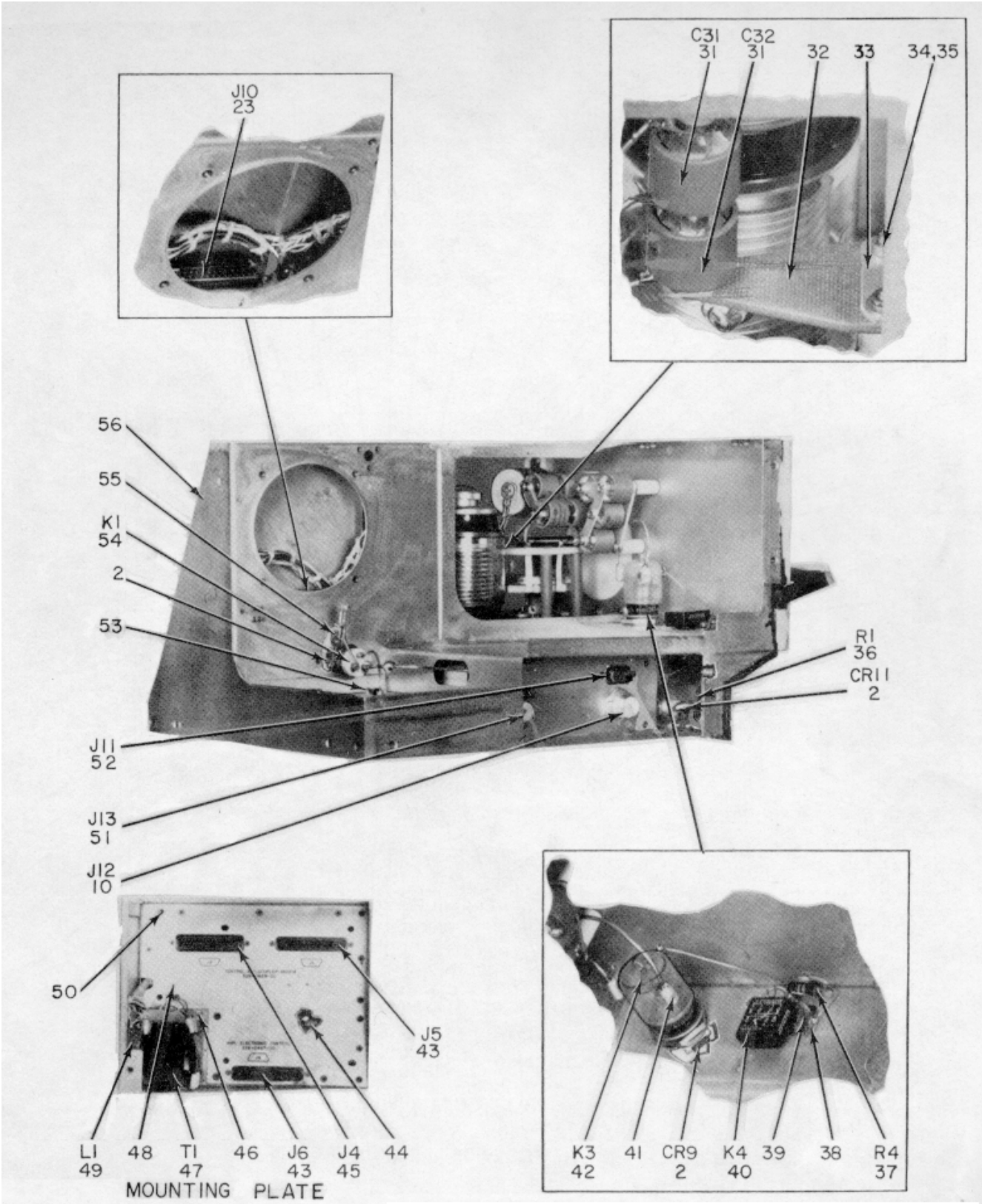
ASSEMBLY VIEW
