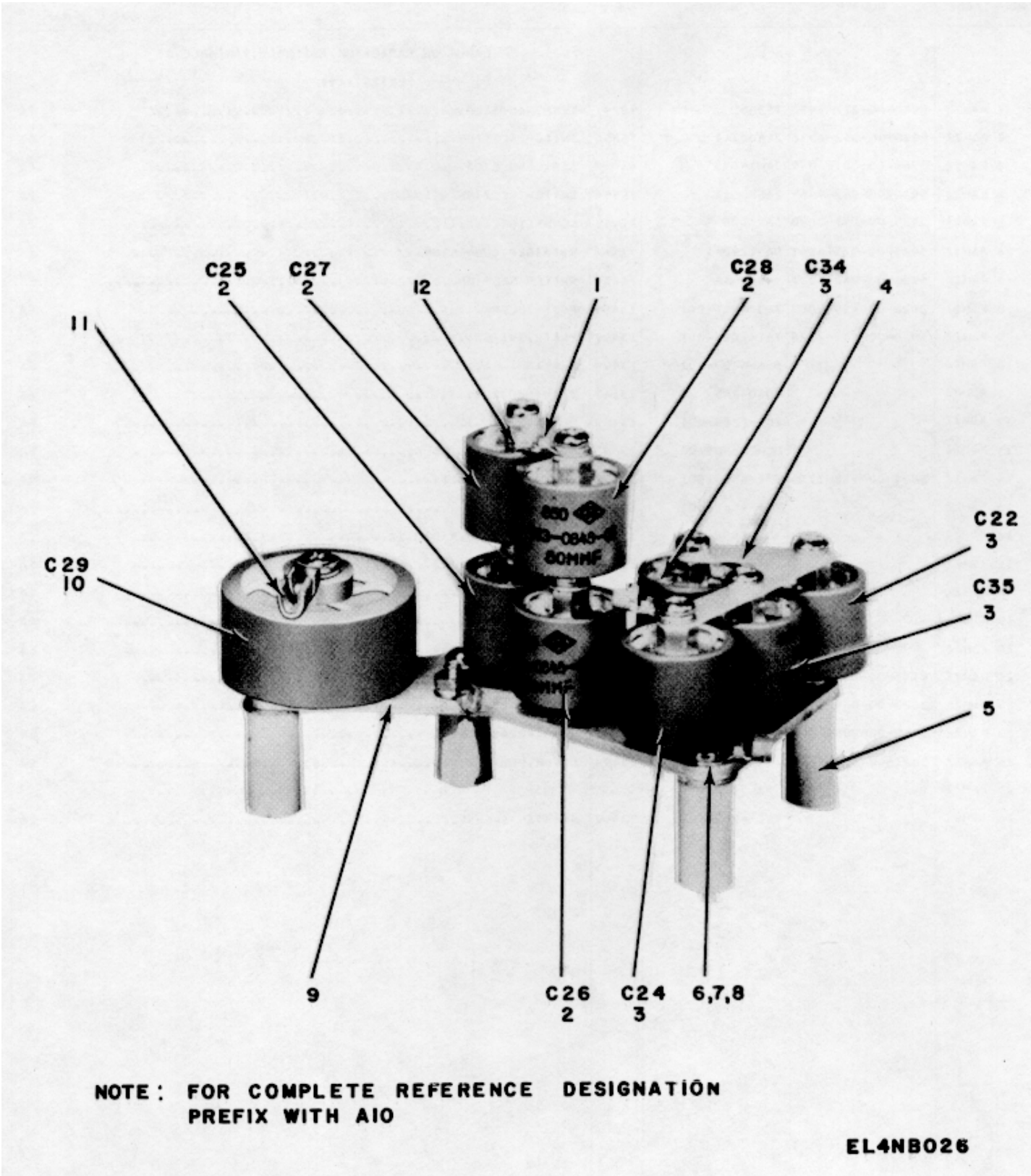
Figure 19. Capacitor Assembly (A10).
