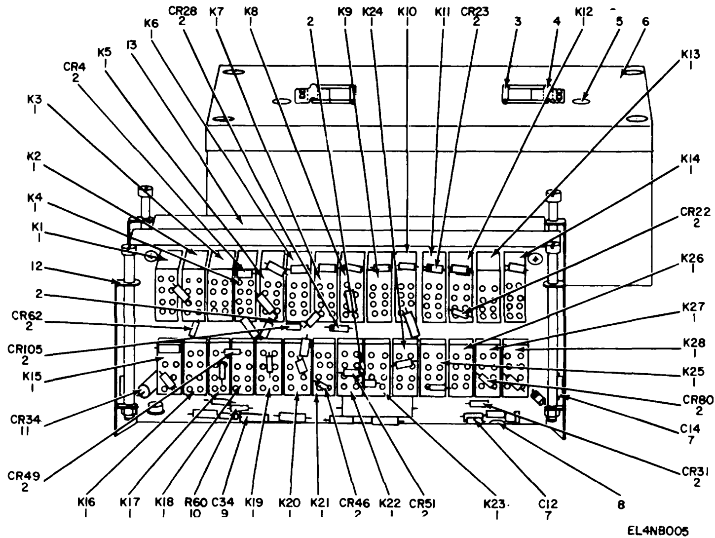
FRONT VIEW, PARTS LOCATION
