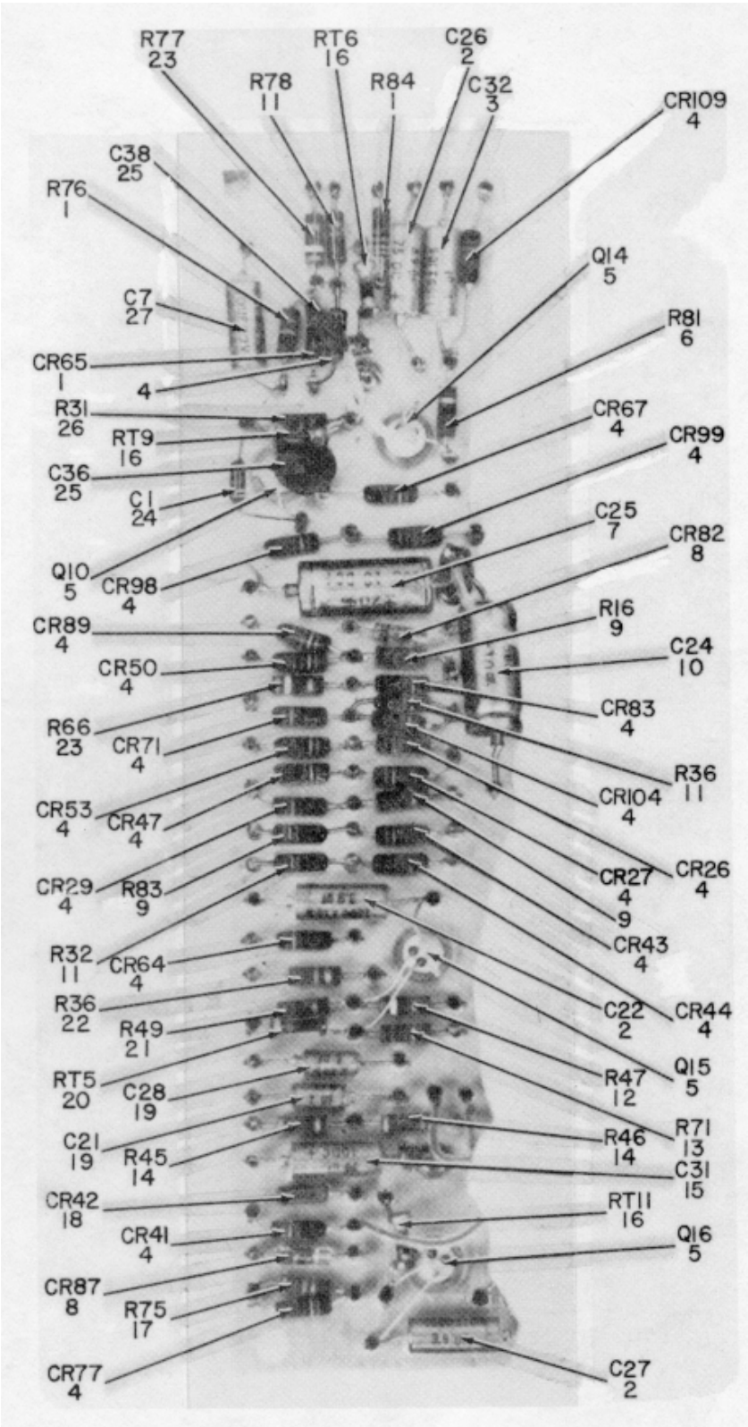
PARTIAL VIEW (LEFT SIDE)
