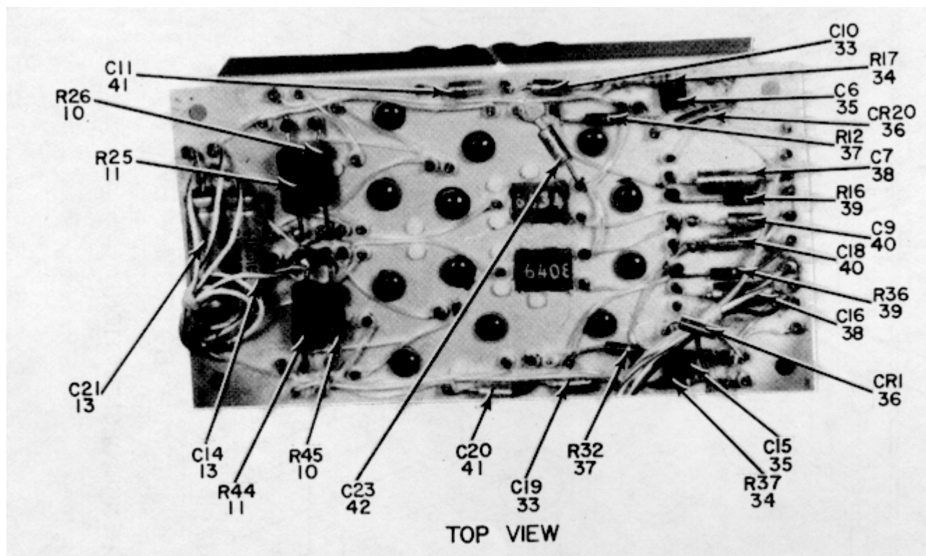
Figure 10. Amplifier, Electronic Control (A3) Terminal Board (Sheet 2 of 2).
