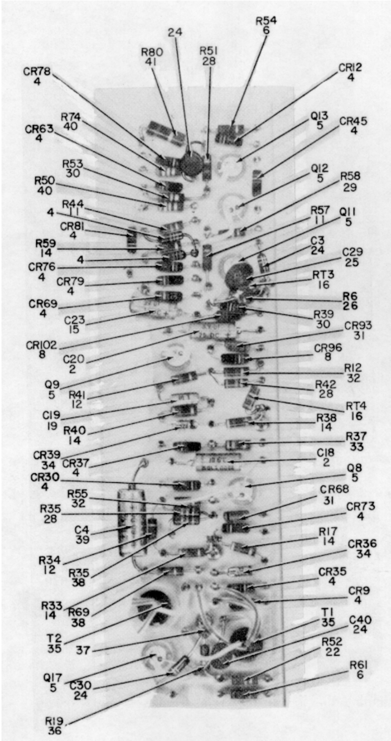
PARTIAL VIEW (RIGHT SIDE)
