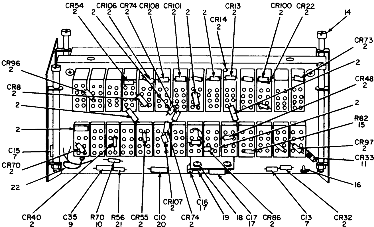
FRONT VIEW, ADDITIONAL PARTS LOCATION
