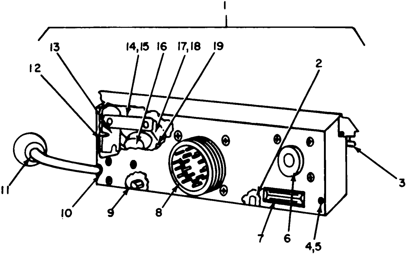
Figure 2. Chassis, electrical equipment (A1) Connector Adapter Assembly.
