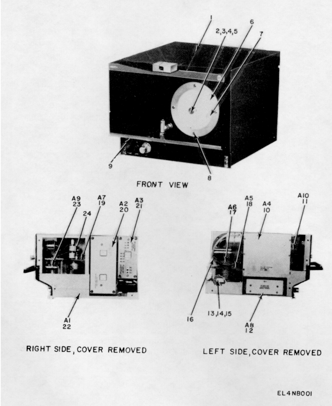
Figure 1. Coupler, Antenna CU-1658/A and CU-1658A/A. Coupler, Antenna CU-1669/CRC.
